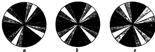
FIG. 126.—A disc b of 24 Mica Sectors under Crossed Nicols, showing Effects at a and c of Introduction of Left- and Right-handed Quartz Plates.
